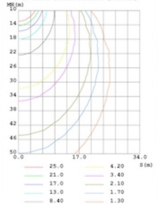
CO PLANE ISOLUX DIAGRAM (UNIT: lx)
